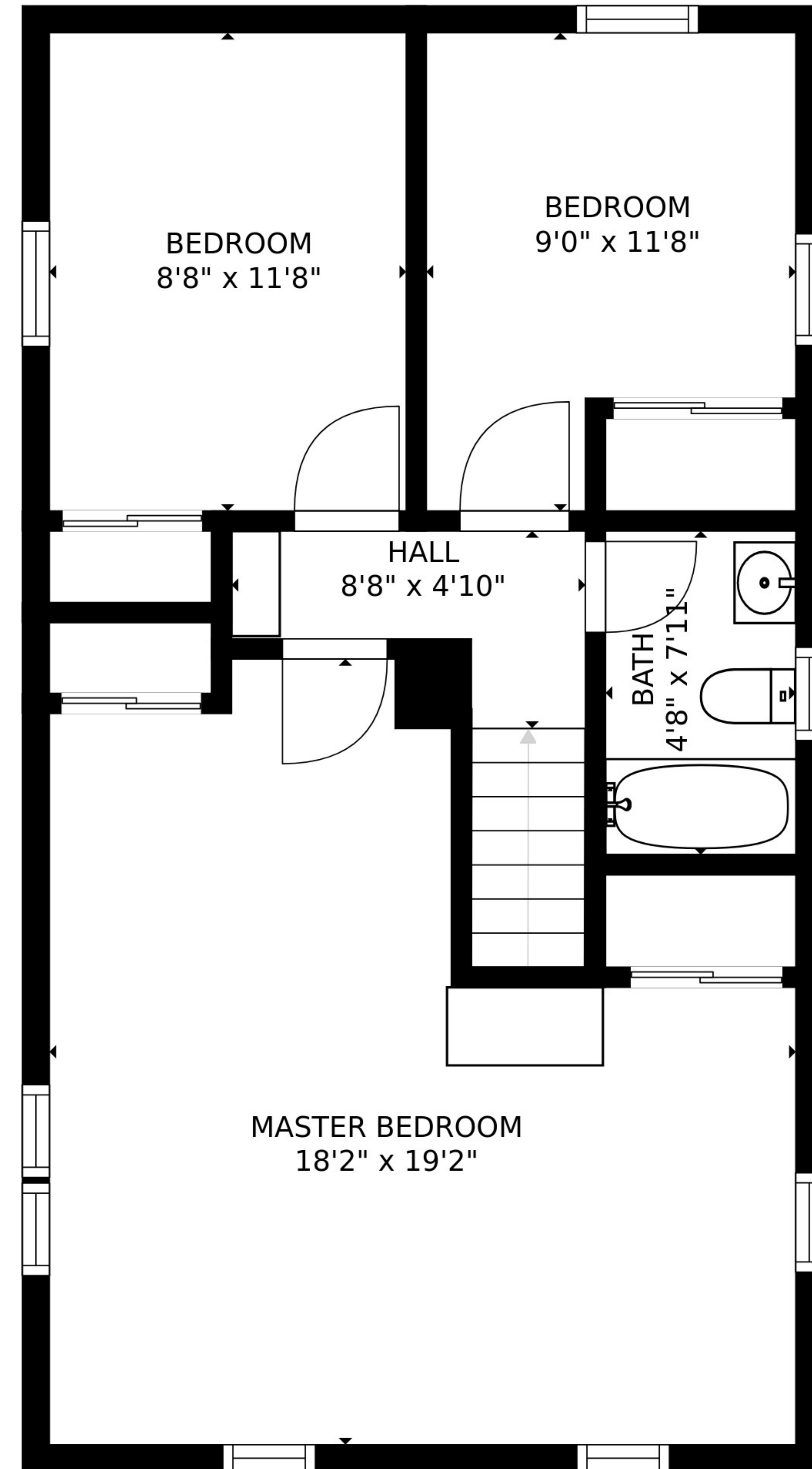
FLOOR 2
